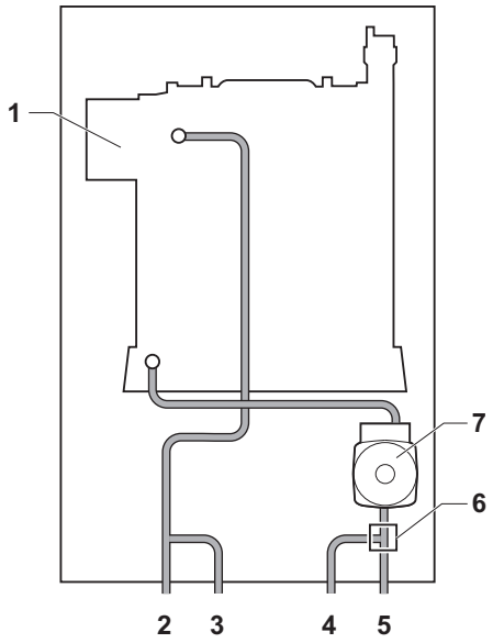
Fig.6 Calenta Ace 35DS
