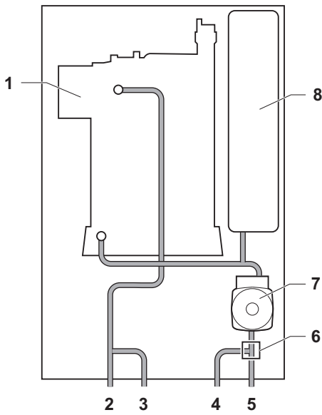
Fig.5 Calenta Ace 15DS - 25DS
