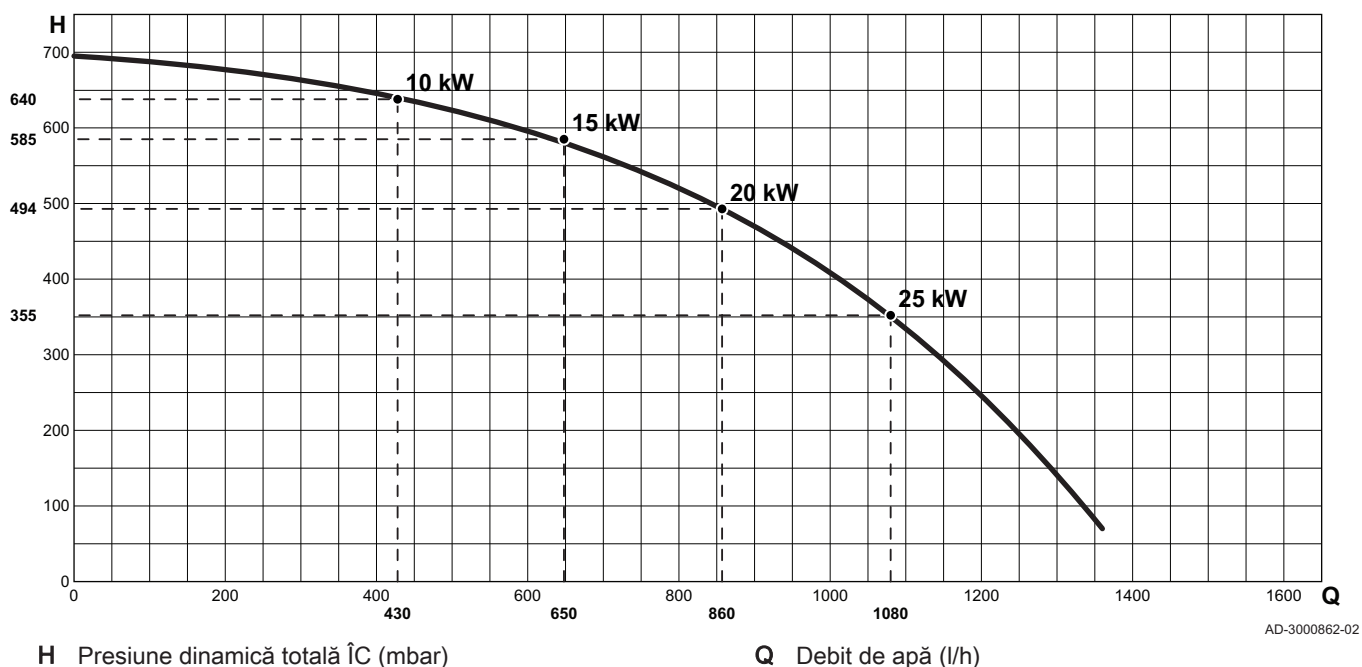
Fig.1 Calenta Ace 15S - 15DS - 25S - 25DS - 28C
