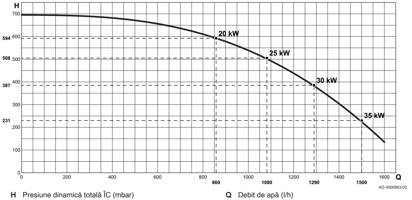
Fig.2 Calenta Ace 35S - 35DS - 40C
